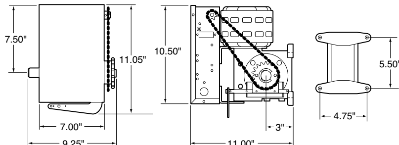
MOUNTING DIMENSIONS
